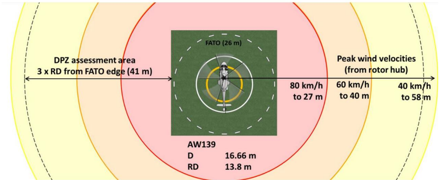
Figure 3: DPZ verses the peak wind velocity data for a AW139 (source: CASA)
