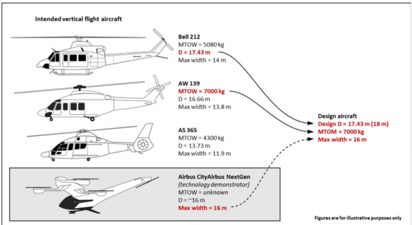
Figure 2: Compiling the design vertical flight aircraft data (source: CASA)
