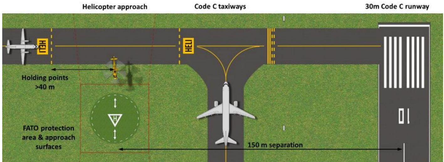
Figure 31: Standalone FATO and separation distances (source: CASA)
