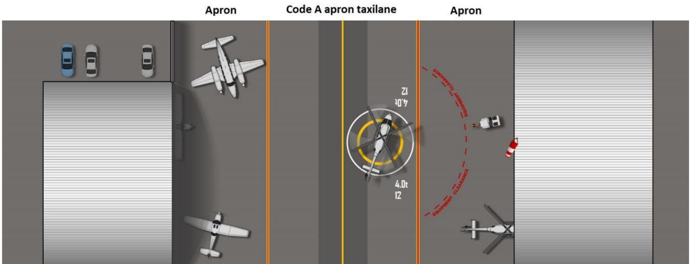
Figure 24: TLOF for a narrow parking area (source: CASA)
