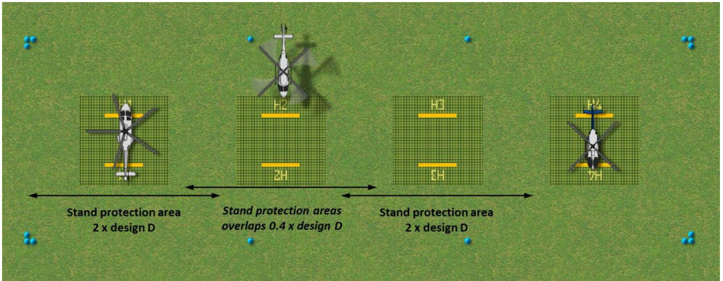
Figure 21: Non-simultaneous air-taxi (natural surface) apron (source: CASA)
