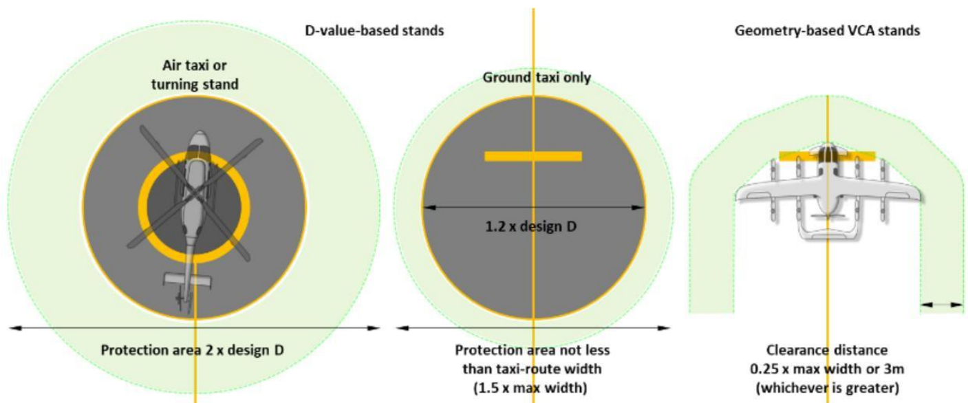
Figure 17: The basic stand geometry for the 3 types of stands (left to right) air-taxi or turning stand, a ground taxi (non-turning) stand and a VCA geometry-based stand (Source: CASA)
