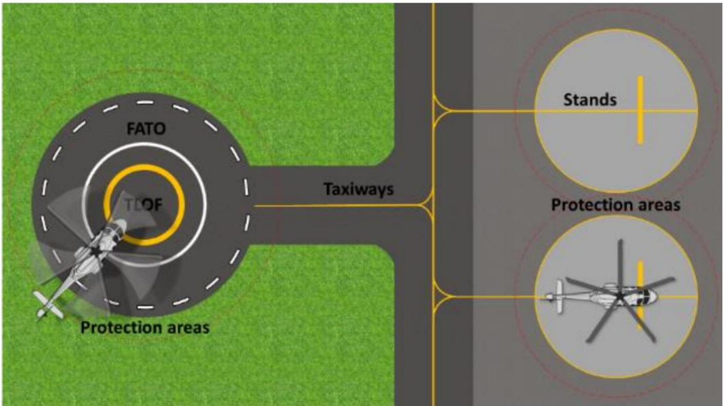
Figure 6: Example of facilities that may be required for vertical flight operations at an aerodrome (Source: CASA.)
