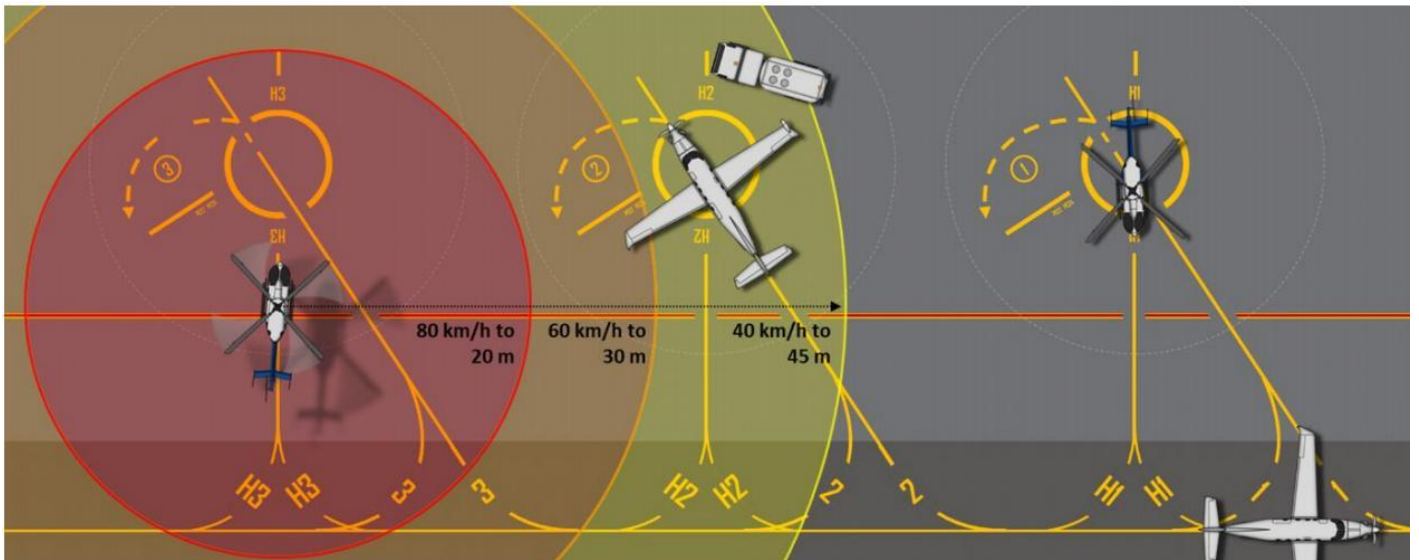
Figure 18: Mixed use apron design (source: CASA)
