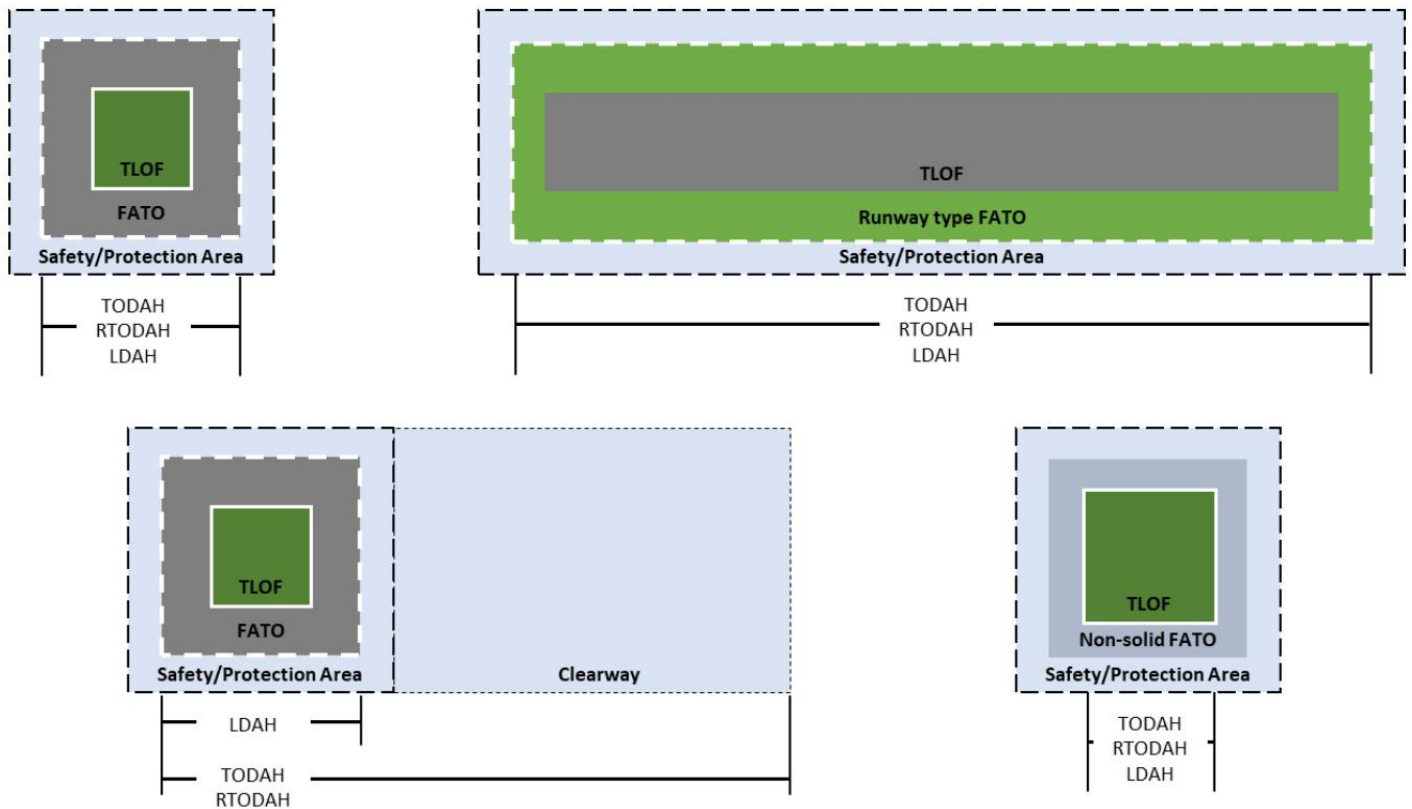
Figure 39: Visual explanation of declared distances for different FATO types. (Source: CASA)
