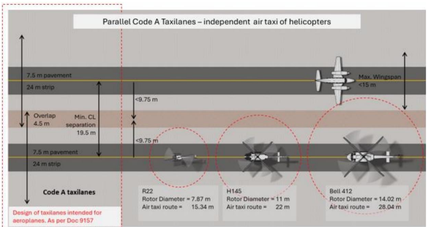
Figure 14: Parallel code A taxilanes and the air-taxi routes for 3 helicopters with a width of less than 15 m (Source: CASA)
