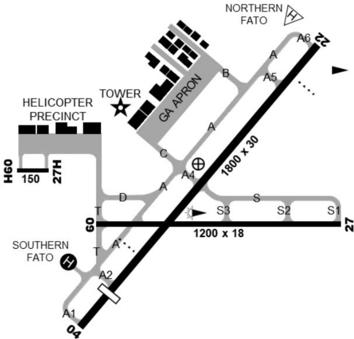
Figure 37: Fictional aerodrome diagram (Source: CASA)
