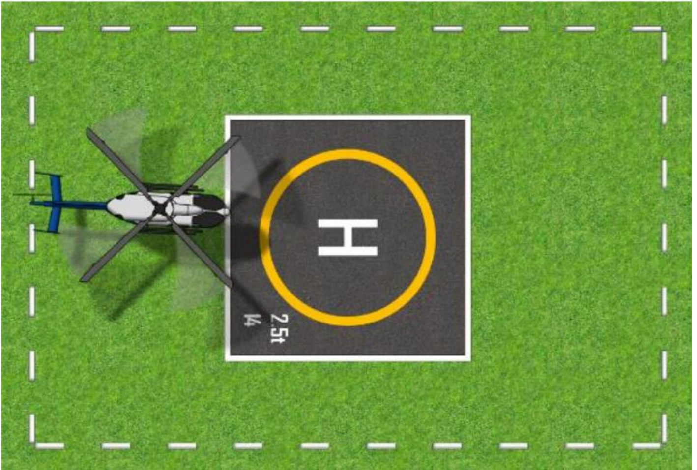
Figure 28: FATO with a TLOF
