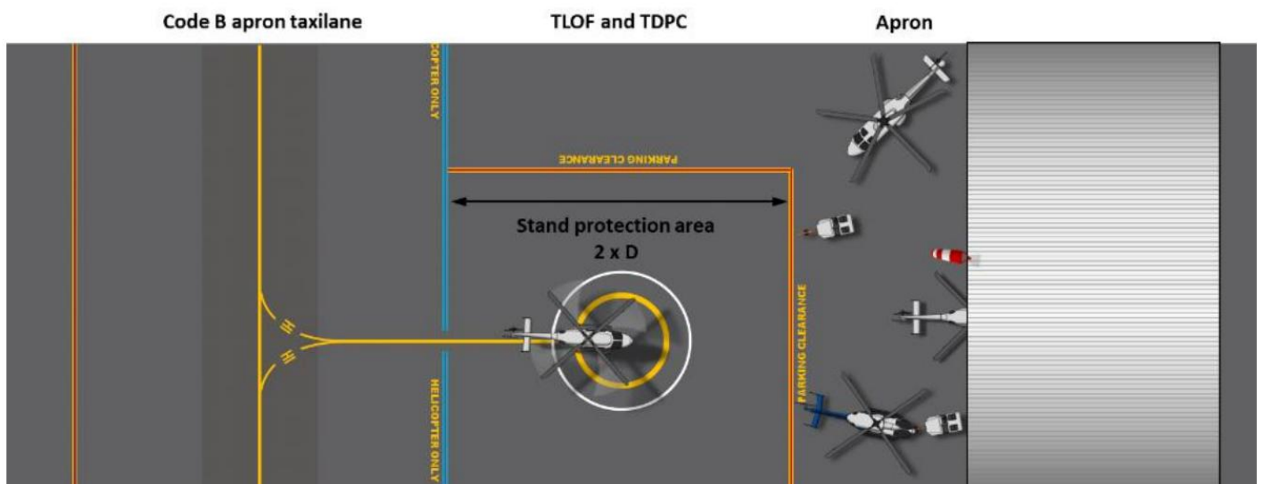
Figure 22: TLOF on an apron (source: CASA)
