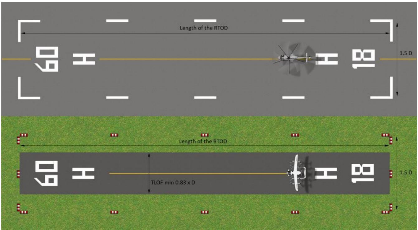
Figure 9: Runway type FATO examples (Source: CASA)
