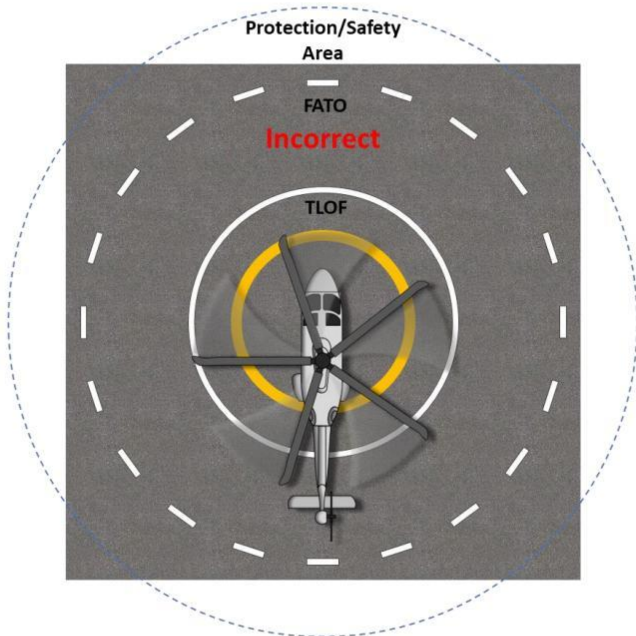
Figure 32: Correct touch down alignment over the TDPC vs incorrect alignment touch down on the "H" marking (source: CASA)
