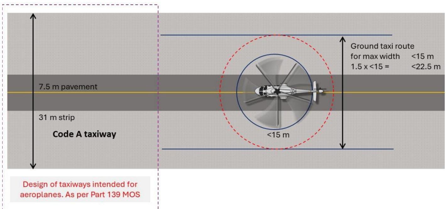
Figure 11: Illustration of a code A taxiway and taxiway strip vs the ground taxi route width for a helicopter of <15 m
