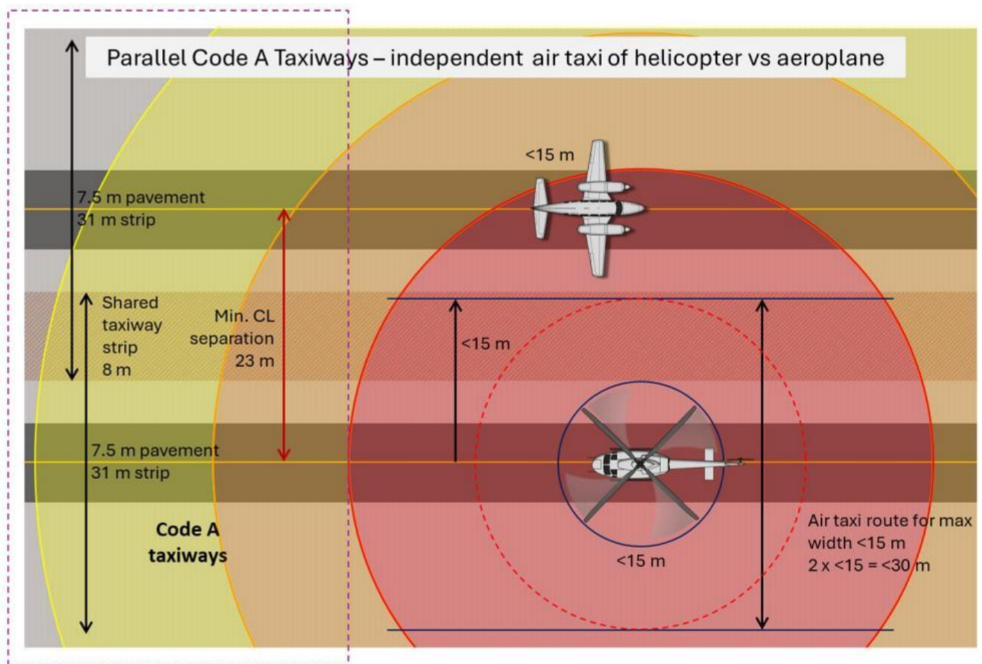
Figure 15: Parallel code A taxiways vs the potential peak wind velocities of a Bell 412 (Source: CASA)
