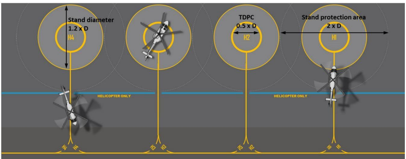
Figure 20: Non-simultaneous air-taxi apron (source: CASA)
