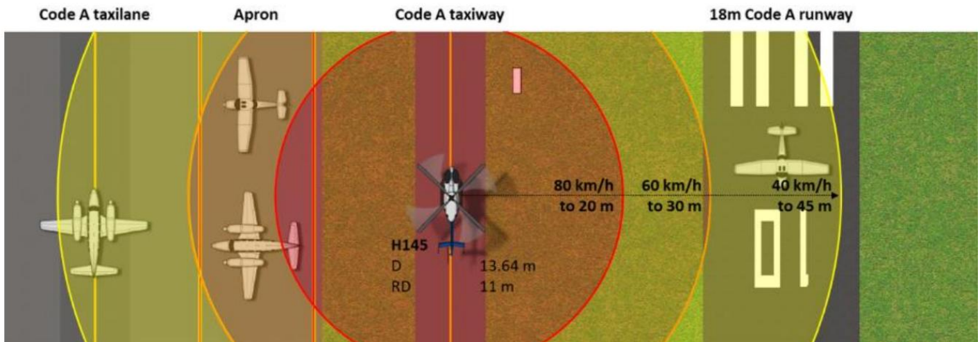
Figure 4: H145 peak wind velocities vs code A separations (source: CASA)
