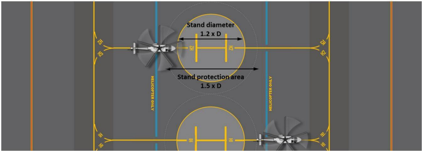
Figure 19: Simultaneous ground taxi apron (source: CASA)
