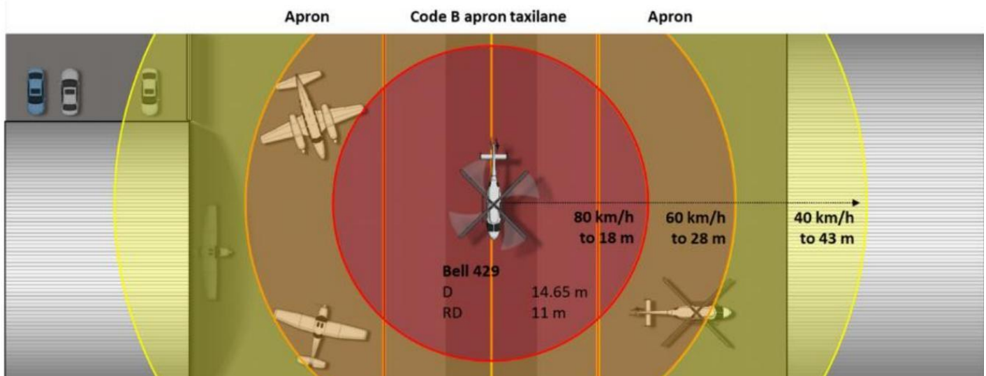
Figure 5: Bell 429 peak wind velocities vs code B separations (source: CASA)
