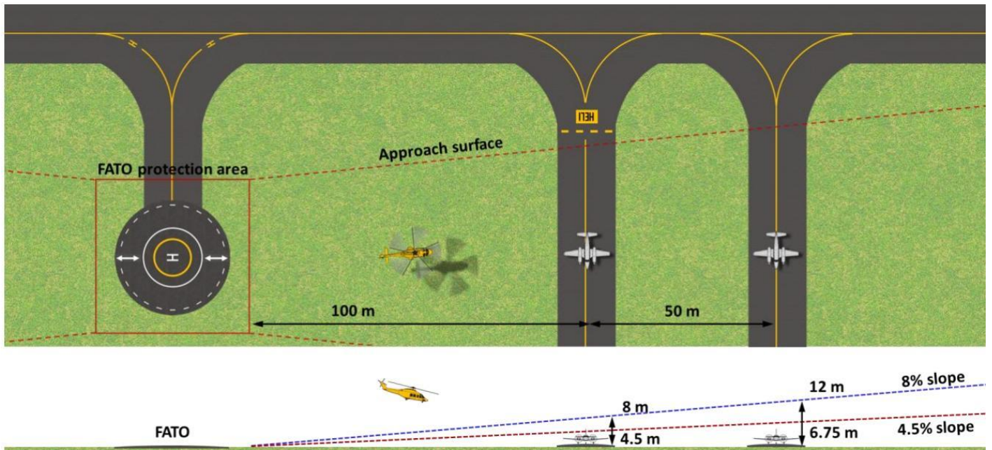
Figure 26: FATO approach and departure slope options (Source: CASA)
