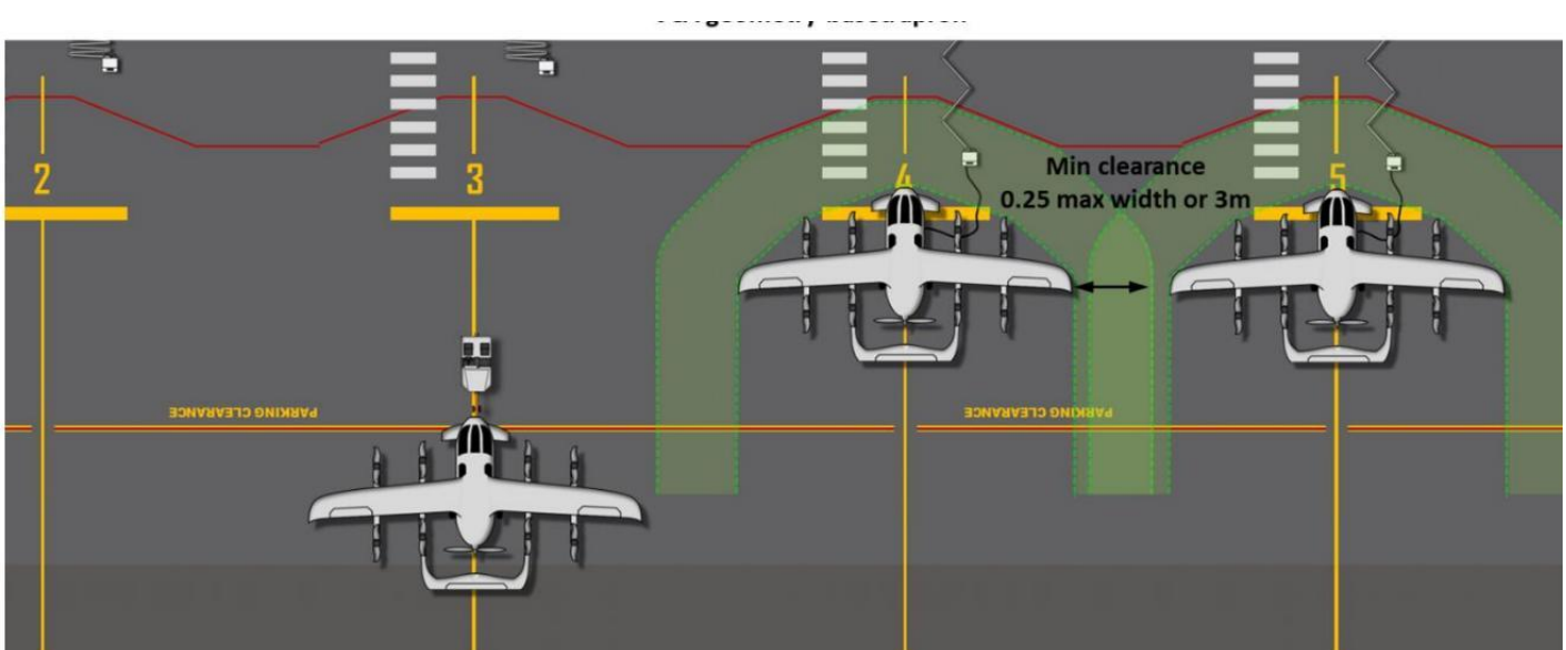
Figure 25: Geometry-based apron (Source: CASA)
