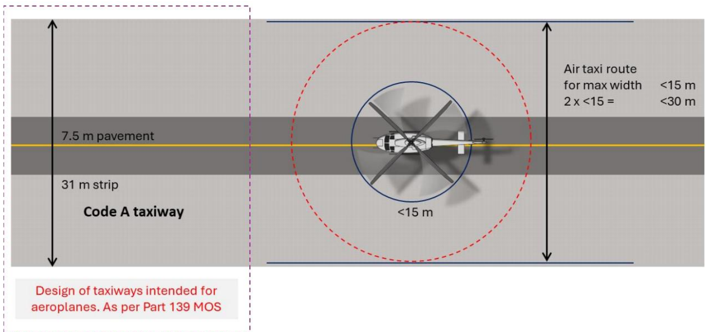
Figure 13: Code A taxiway dimensions vs air-taxi routes (Source: CASA)
