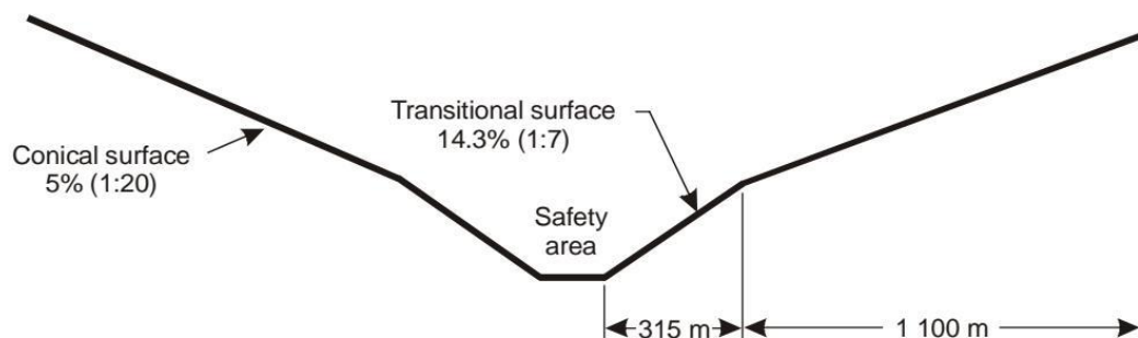
Non-precision approach (end profiles)
