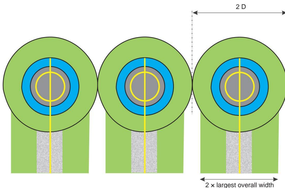
Figure 3-6. Helicopter stands designed for hover turns with air taxi-routes/taxiways — simultaneous operations
