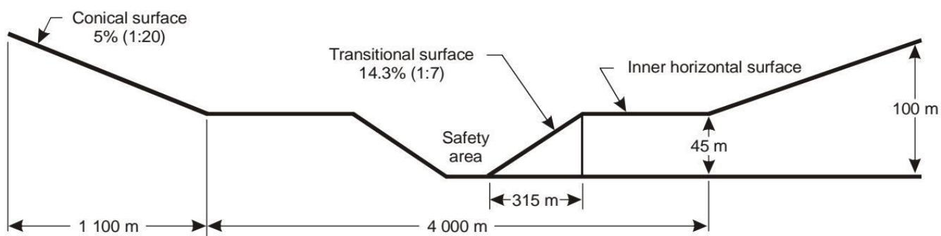
Non-precision approach (end profiles)
