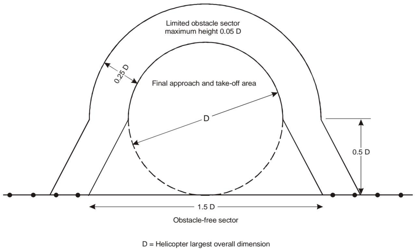
Figure 4-10. Ship's side non-purpose-built heliport obstacle limitation surfaces
