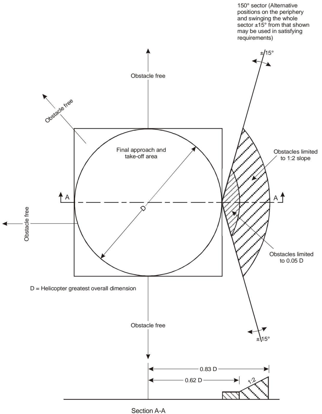
Figure 4-3. Helideck obstacle limitation sectors
