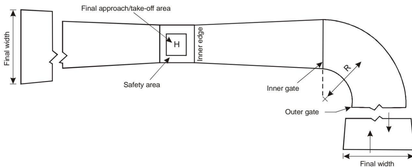
C. Squared final approach and take-off area (curved approach-departure)
