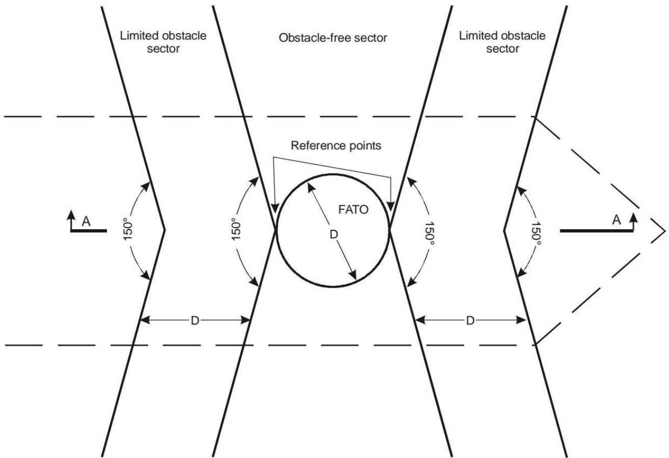
PLAN VIEW
