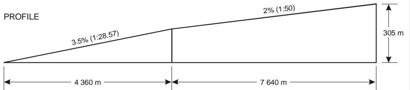
Figure 4-5. Take-off climb surface for instrument FATO
