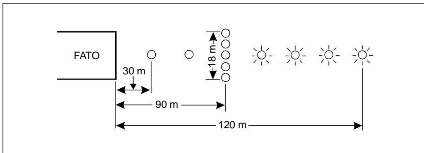
Figure 5-10. Approach lighting system
