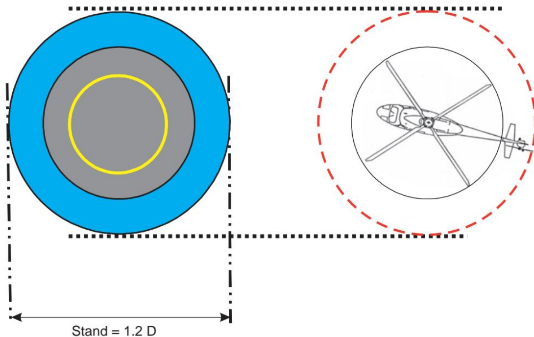
Figure 3-4. Helicopter stand
