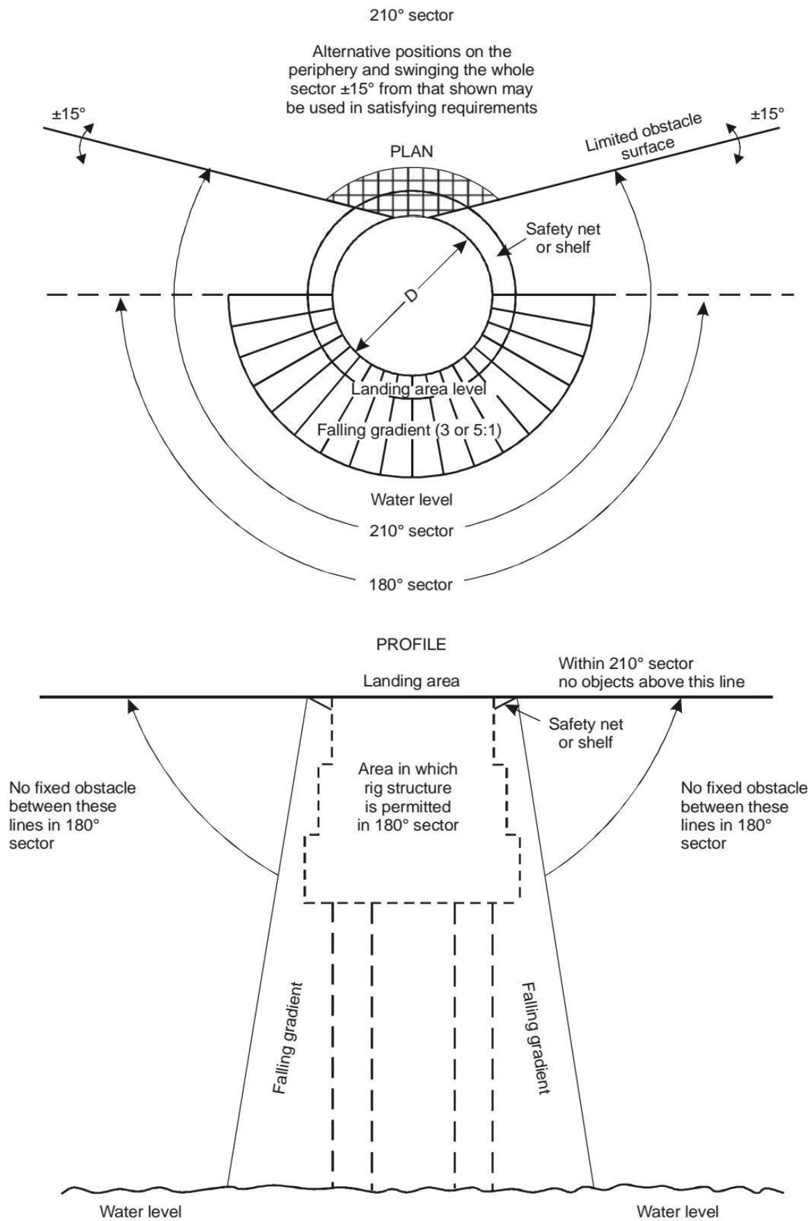
Figure 4-2. Helideck obstacle-free sector
