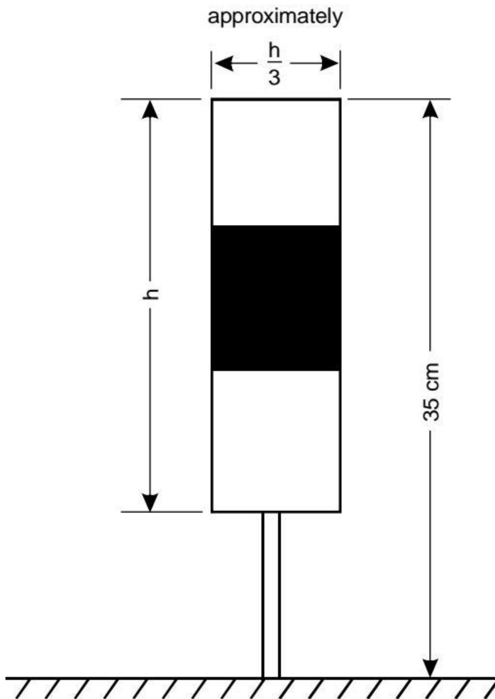
Figure 5-6. Air taxiway marker
