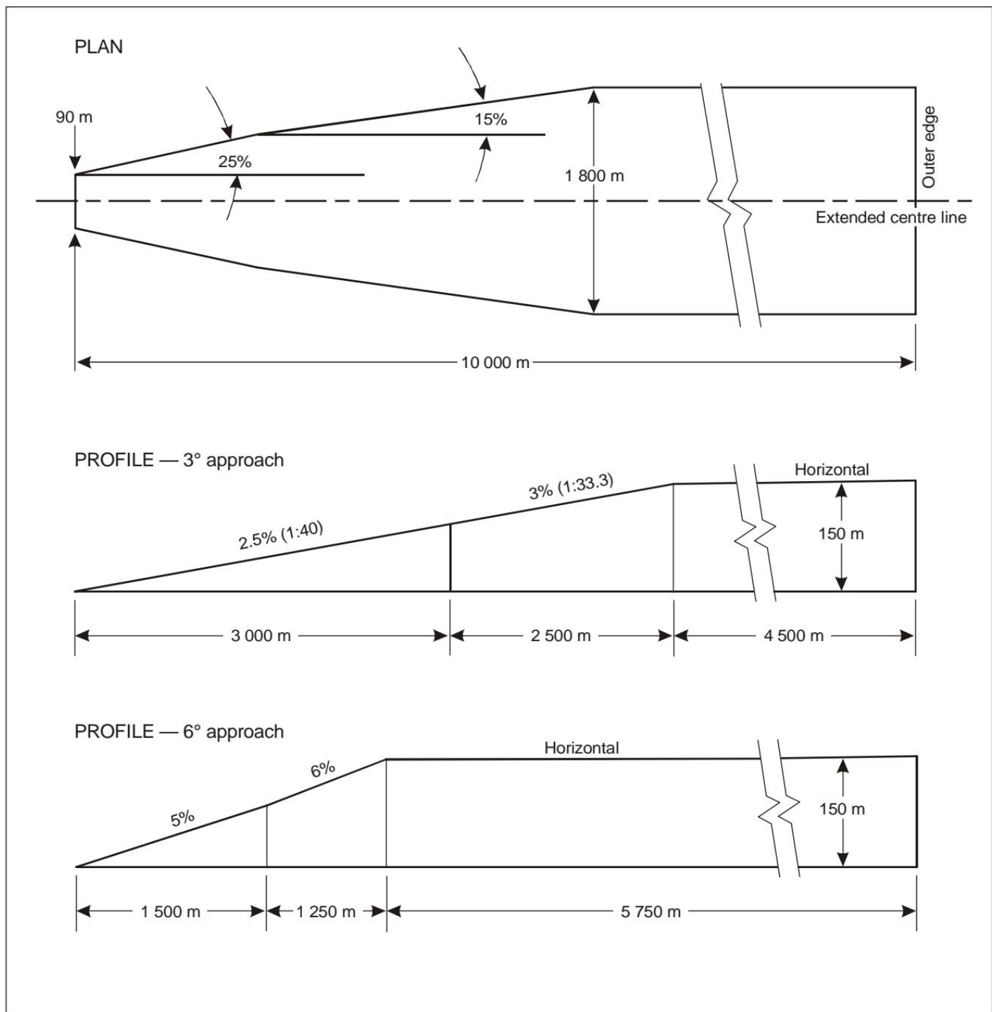
Figure 4-6. Approach surface for precision approach FATO
