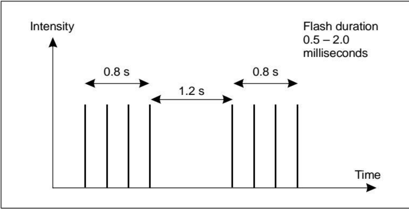
Figure 5-8. Heliport beacon flash characteristics
