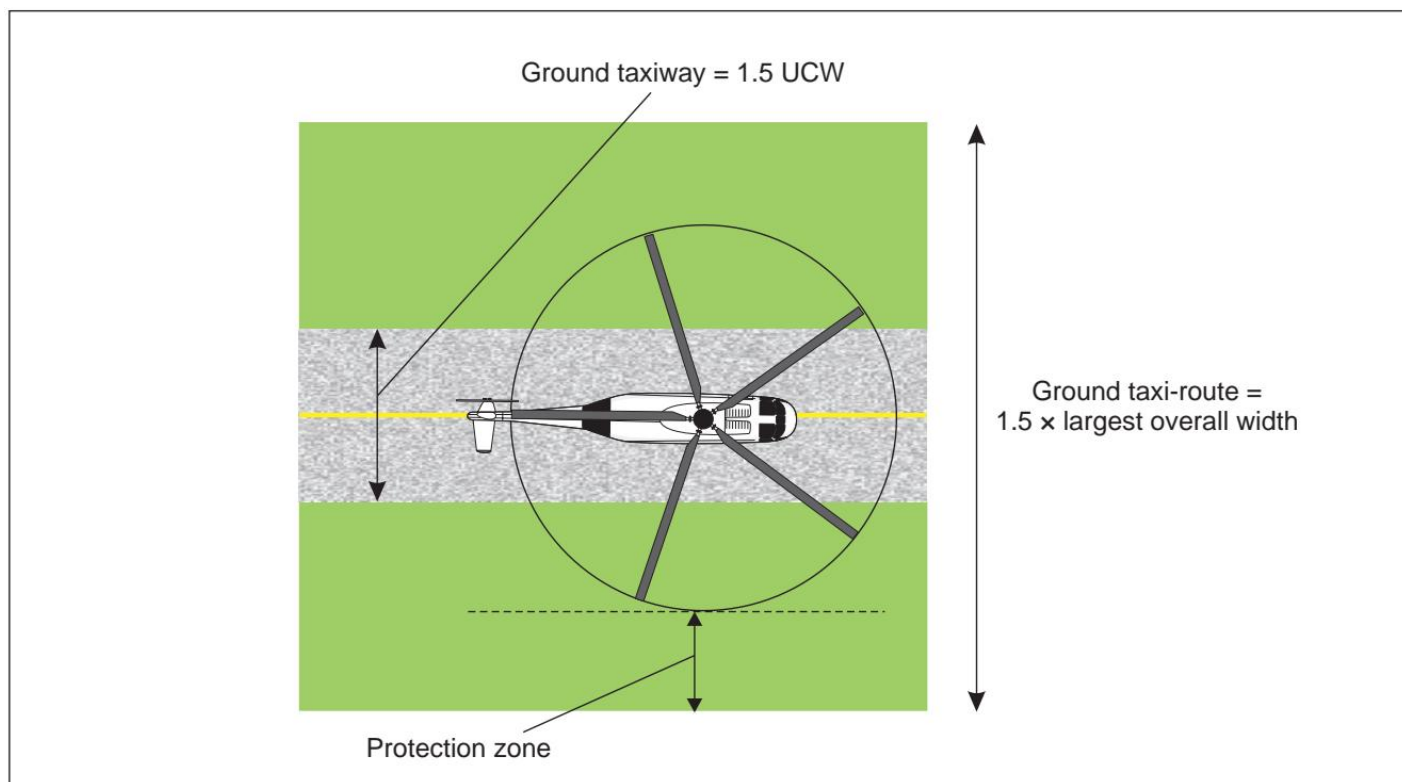
Figure 3-2. Ground taxi-route
