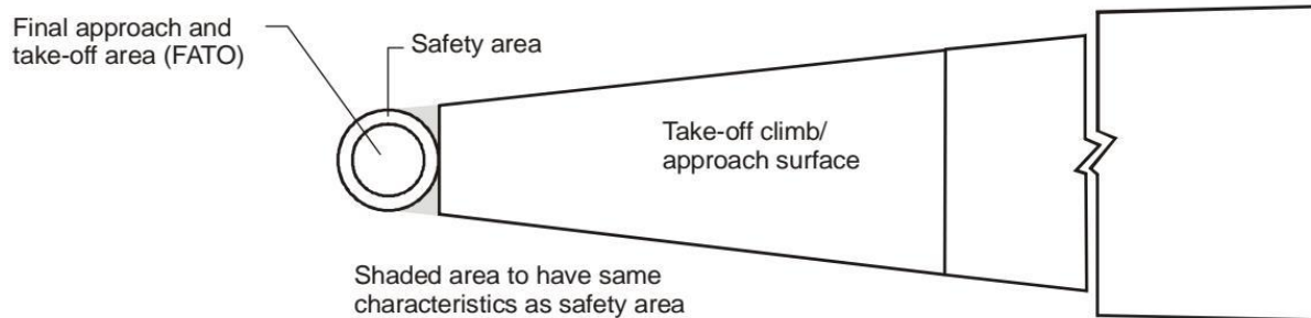
A. Circular final approach and take-off area (straight approach-departure)
