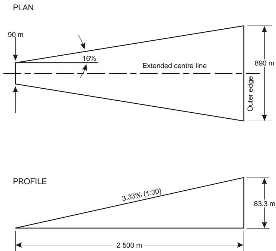
Figure 4-7. Approach surface for non-precision approach FATO
