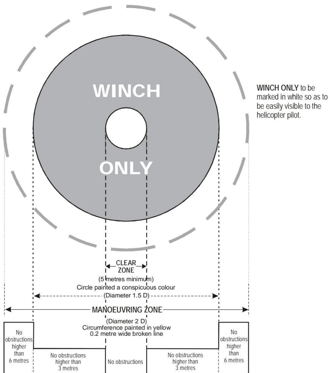
Figure 4-11. Winching area of a ship
