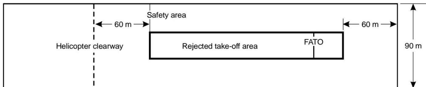
Figure 3-1. Safety area for instrument FATO
