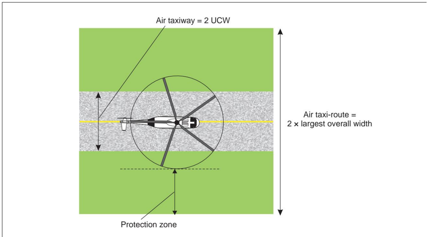
Figure 3-3. Air taxi-route
