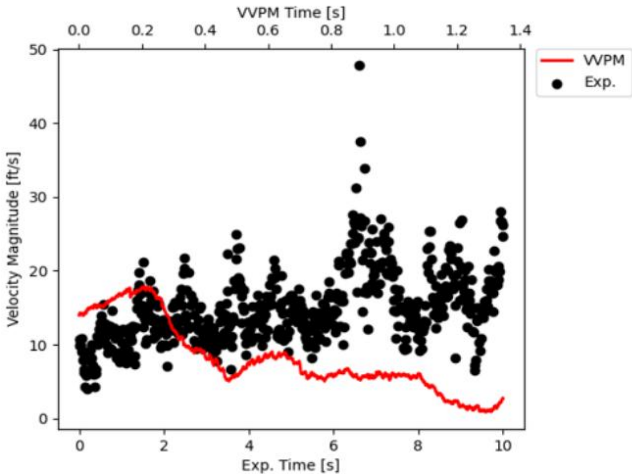
Figure 25. Tethered Test Case Correlation—Time Histories of Velocity of Magnitudes
