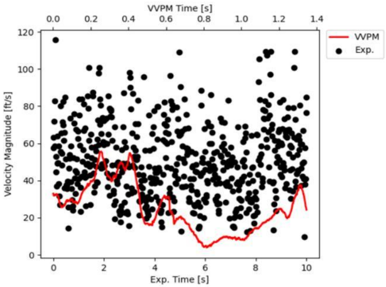
(c) Sensor A2-S30
