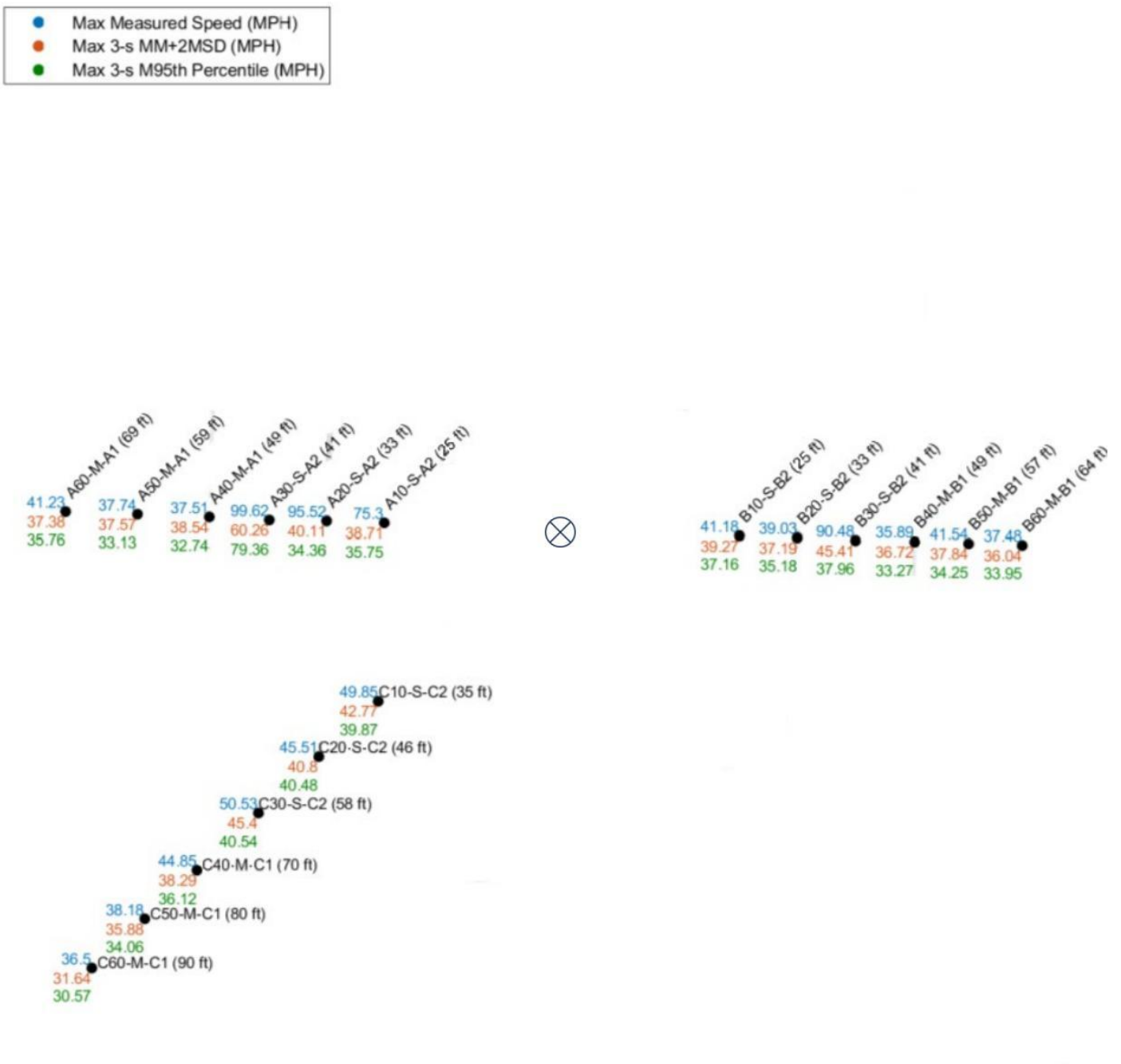
Figure 26. eVTOL #3 Maximum Velocity Recorded at Each Sensor Across All Surveys in Plan View
