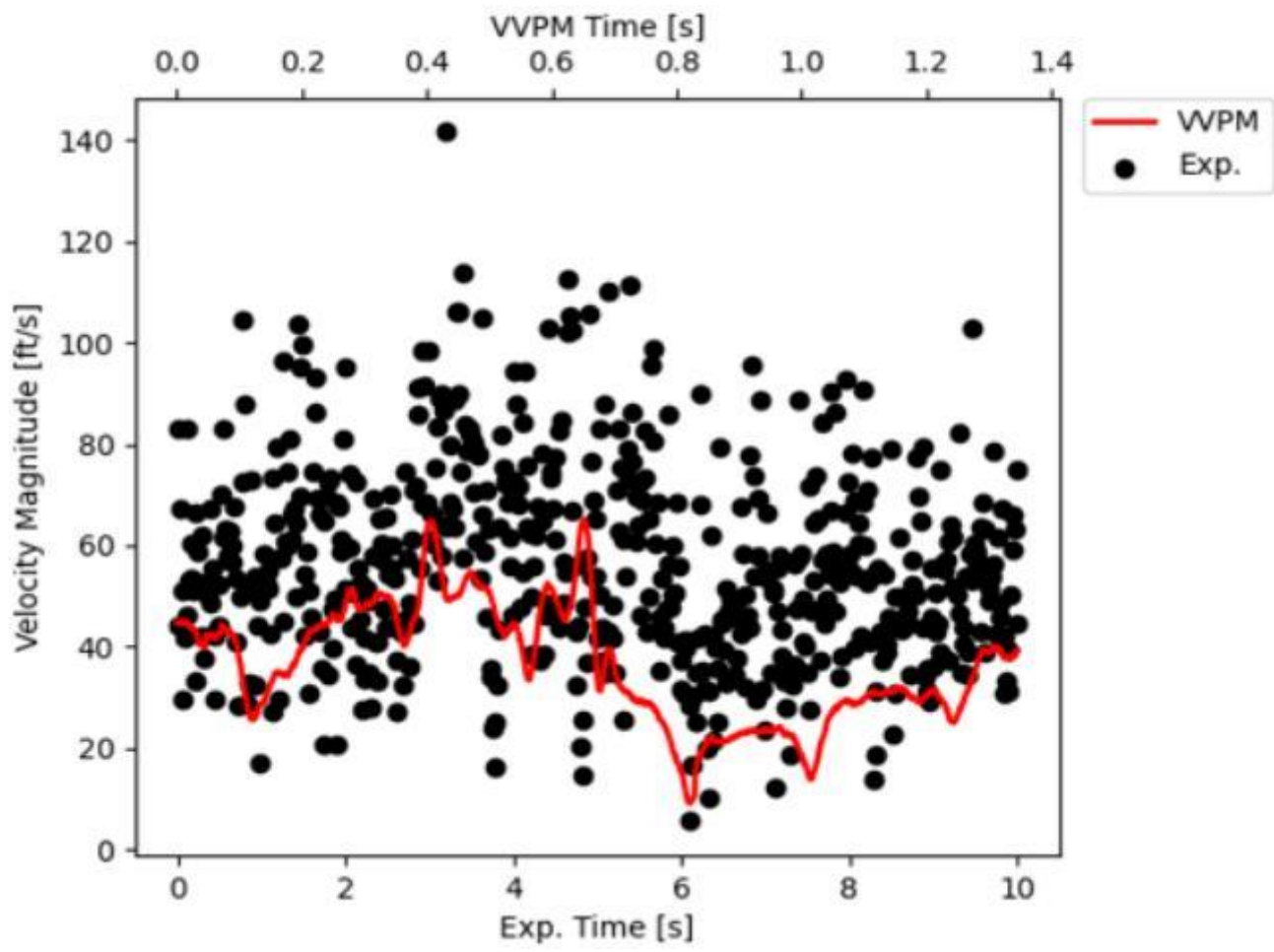
(a) Sensor A2-S10
