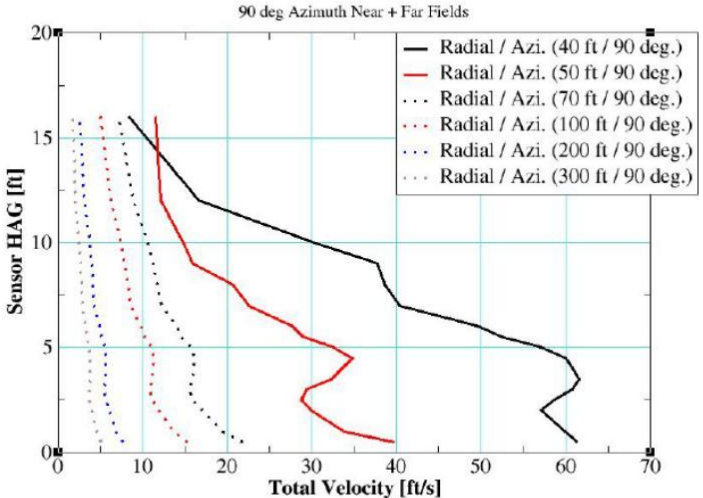
Figure 31. Velocity Profile at 90^\circ Radial
