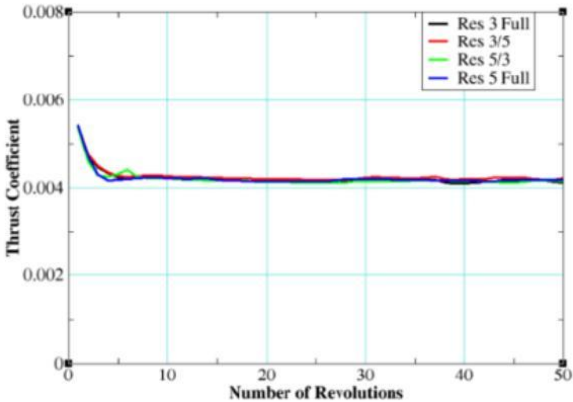
(b) Simulation Convergence for Different Resolutions
