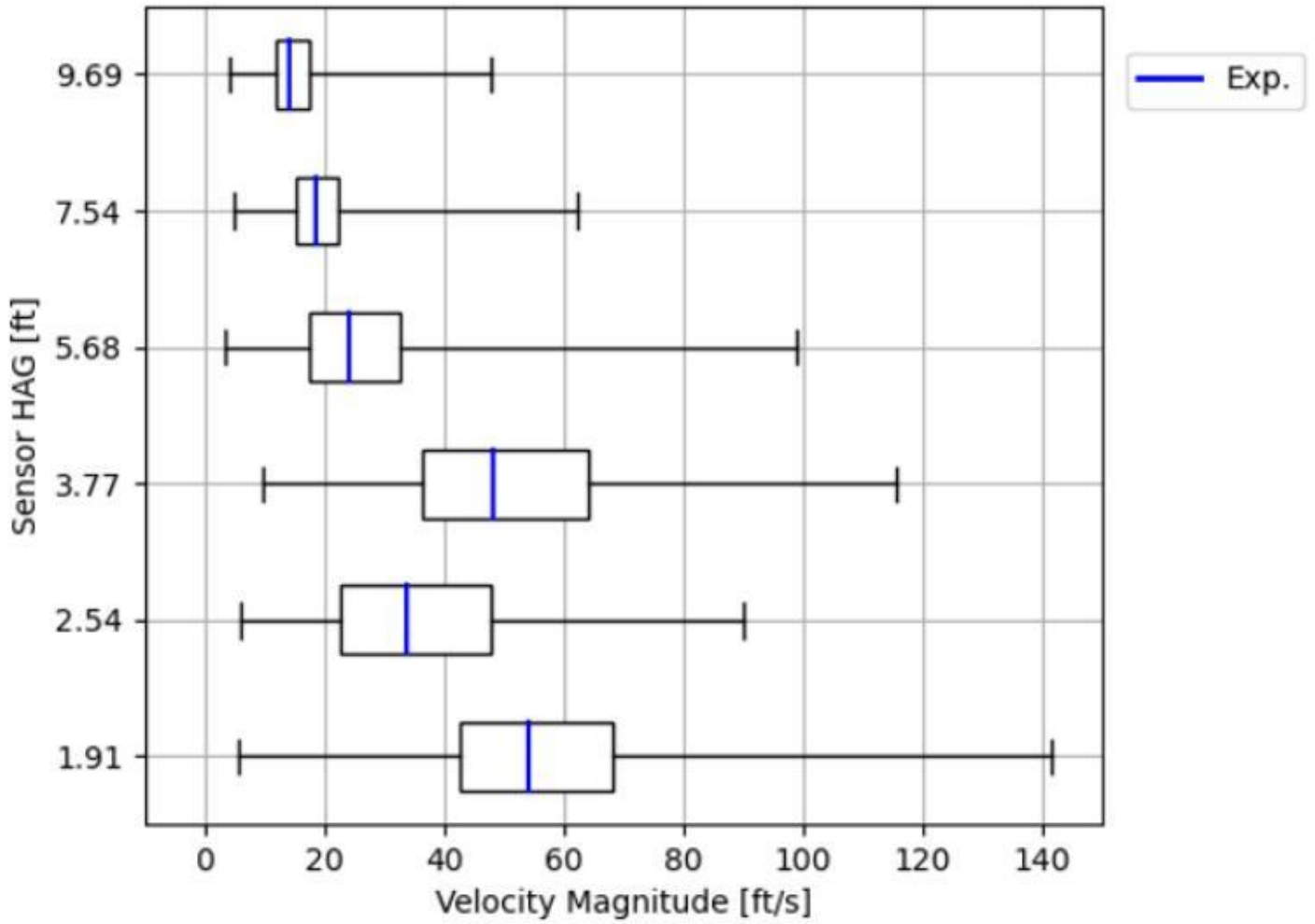
Figure 24. Tethered Test Case Correlation—Boxplots of Velocity Magnitude
