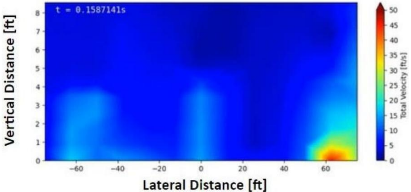
Figure 8. eVTOL #1 Modeled Total Velocity at 69 ft
