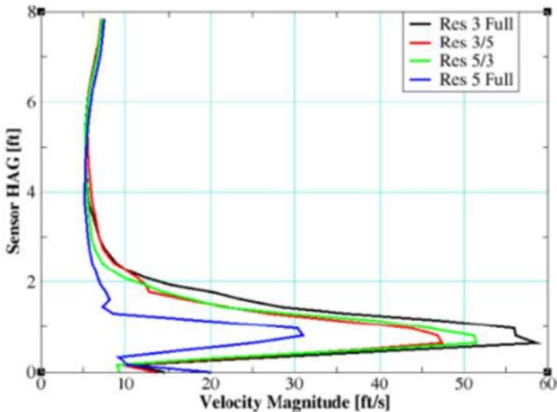
(c) Total Velocity Prediction for Different Resolutions
