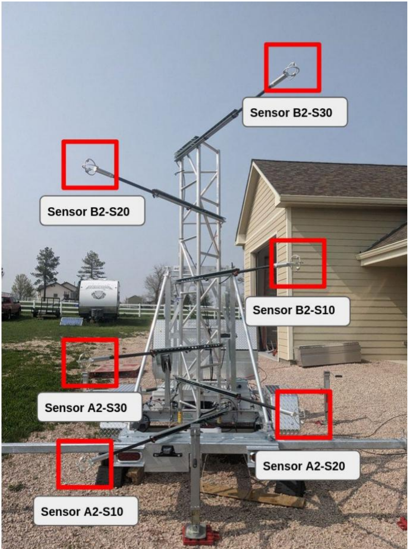
Figure 23. Vertical Array Sensor Configuration
