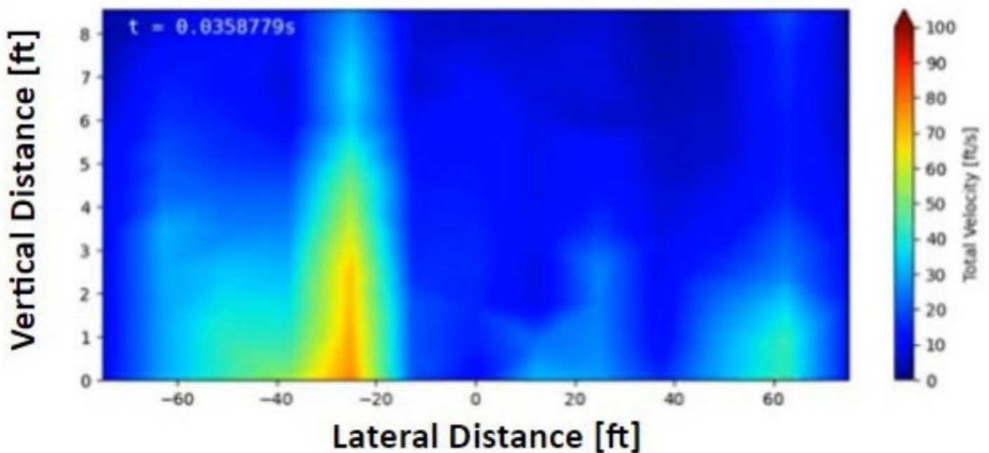
Figure 7. eVTOL #1 Modeled Total Velocity at 46 ft
