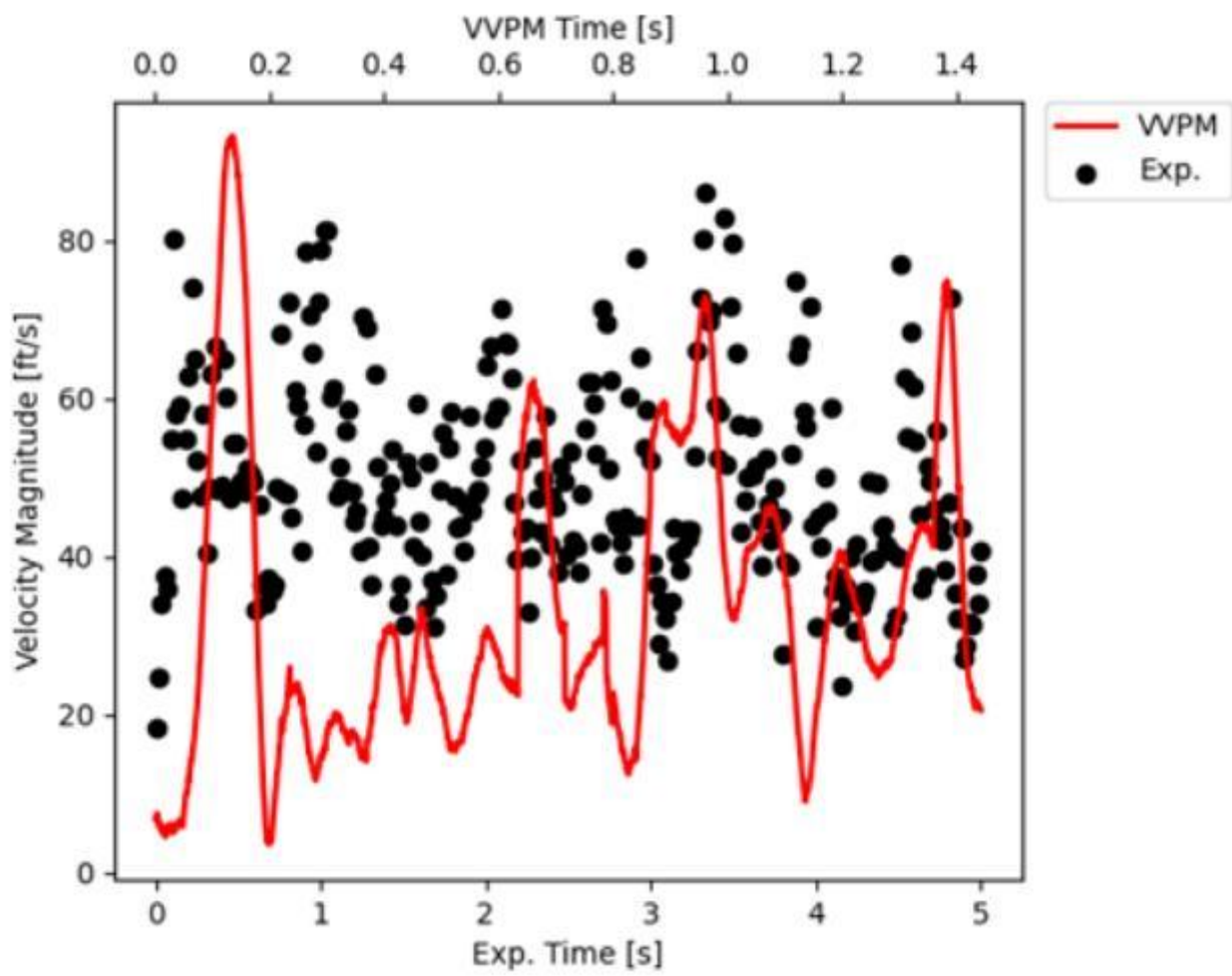
(b) Time History of Velocity
