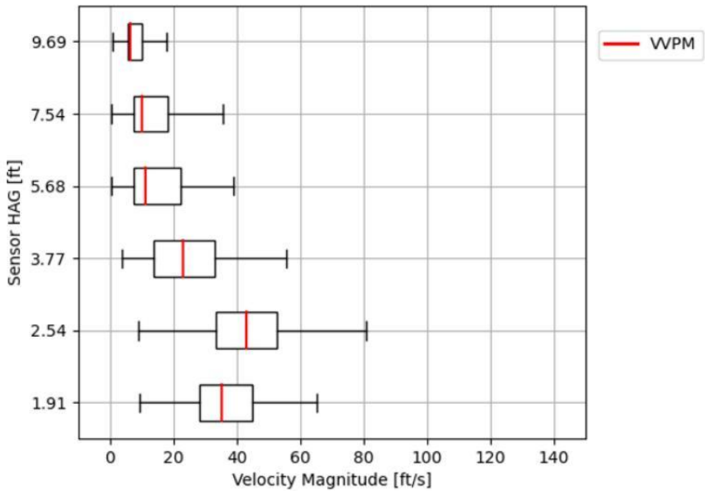
(a) Elevated Thrust Setting (VVPM Simulation)
