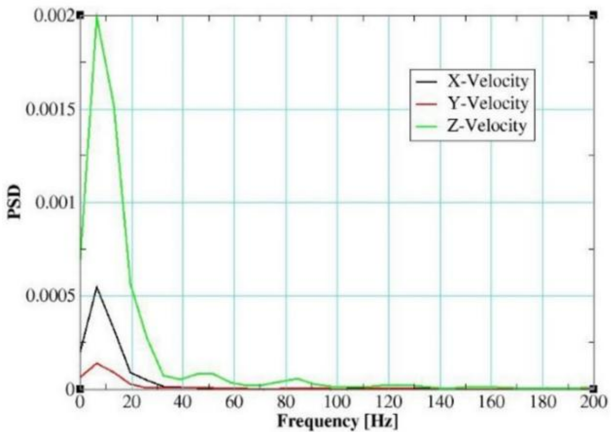
Figure 1. Example Wind Velocity and Blade Frequency Modeled
