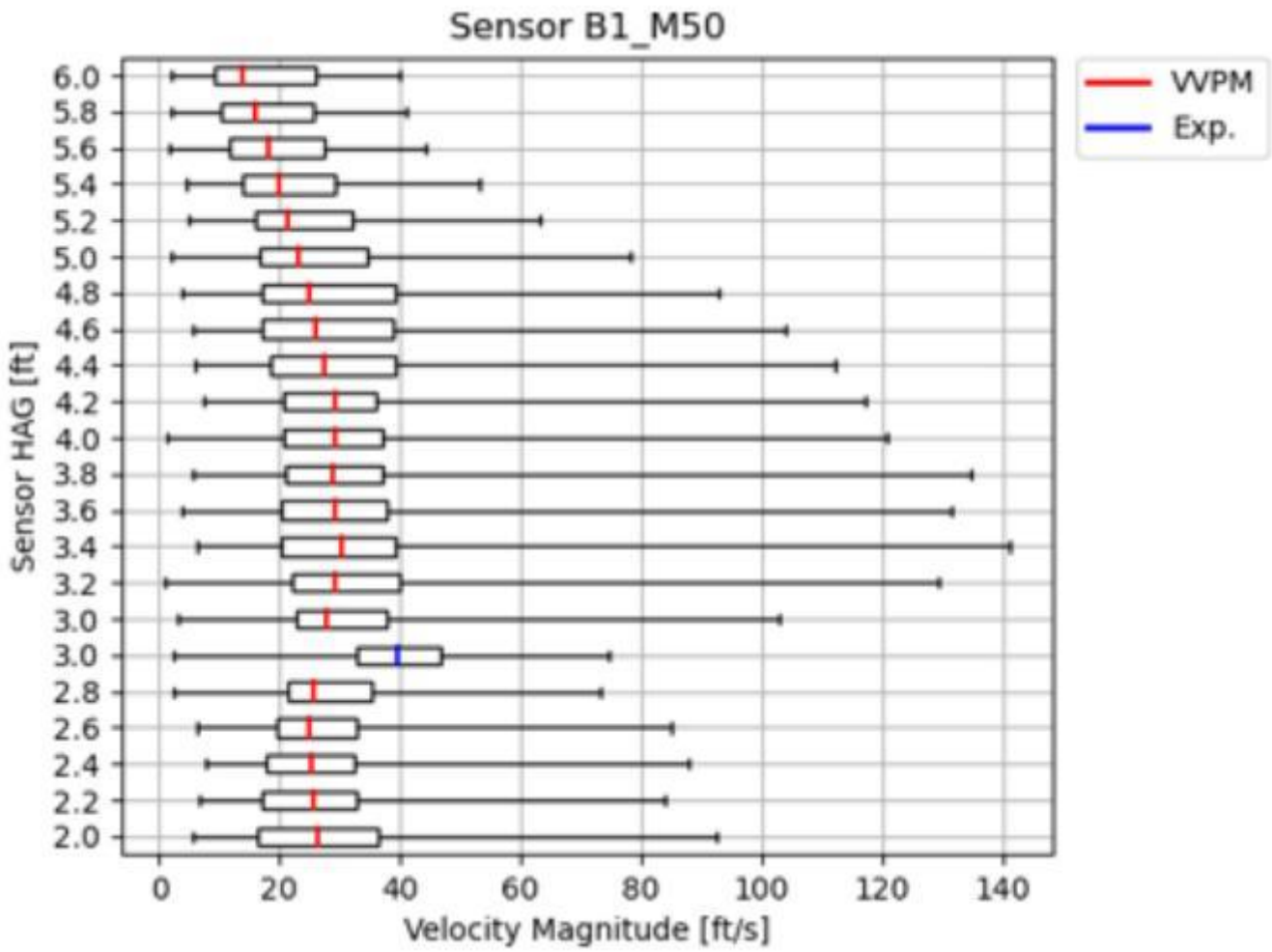
(a) Boxplot of Velocity Magnitude
