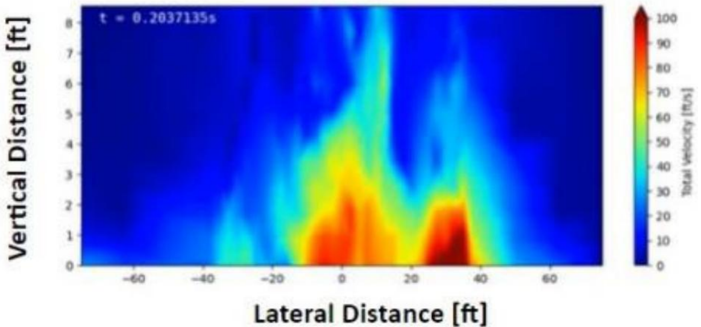
Figure 6. eVTOL #1 Modeled Total Velocity at 23 ft
