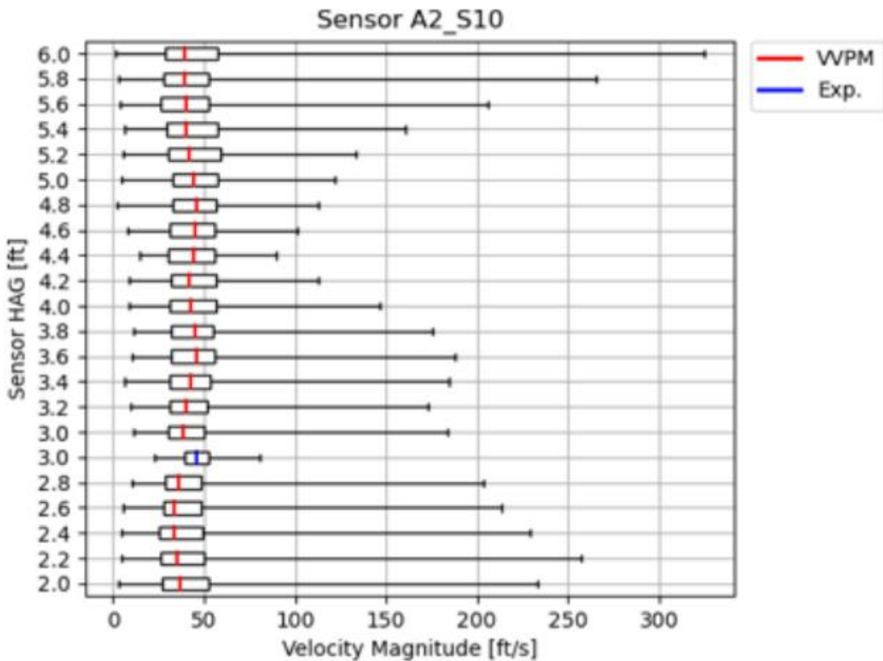
(a) Boxplot of Velocity Magnitude
