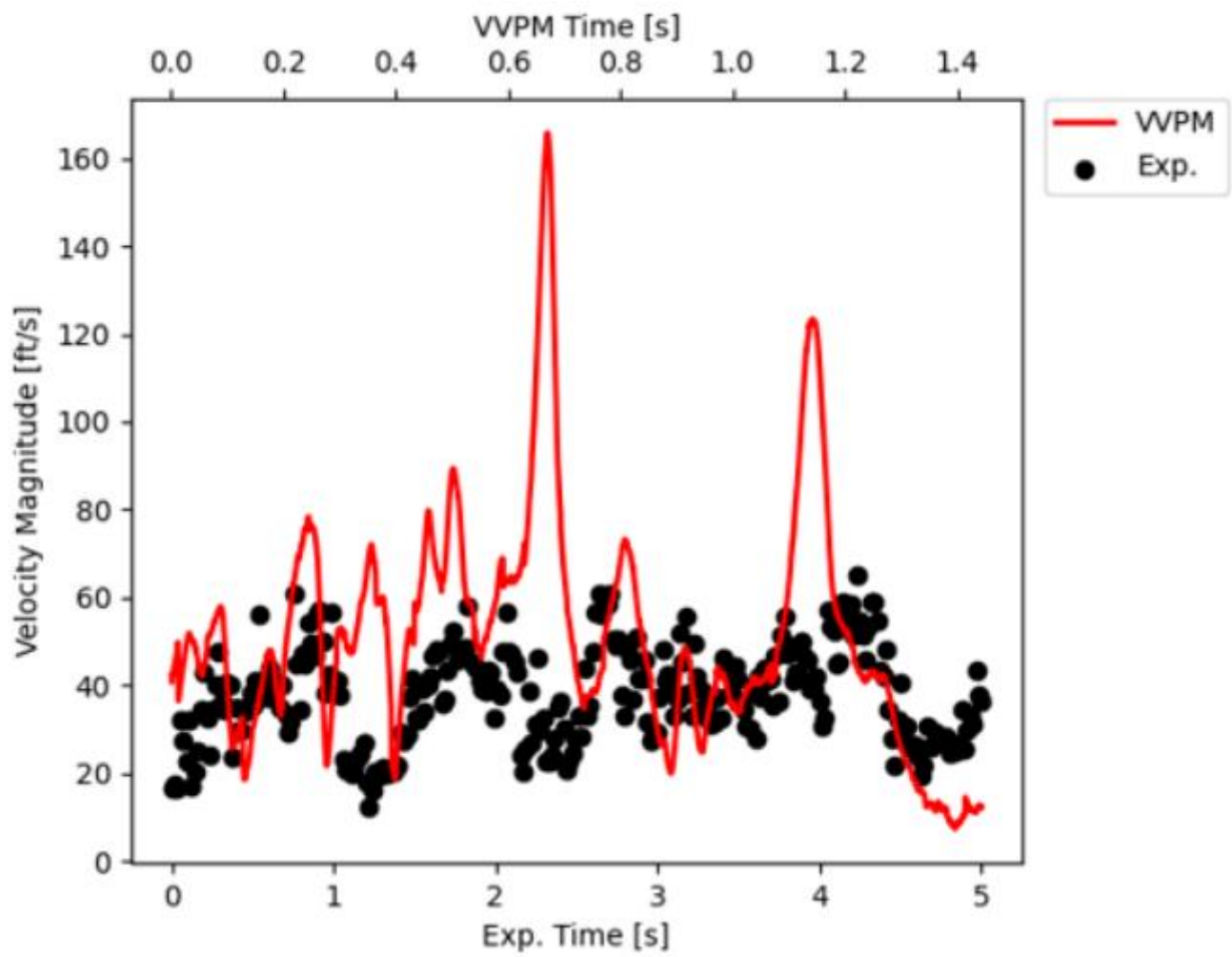
(b) Time History of Velocity
